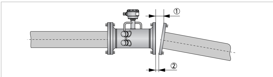
Figure 3-6: Flange deviation
